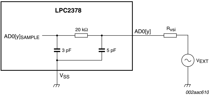
Fig 5. Suggested ADC interface - LPC2378 AD0[y] pin
