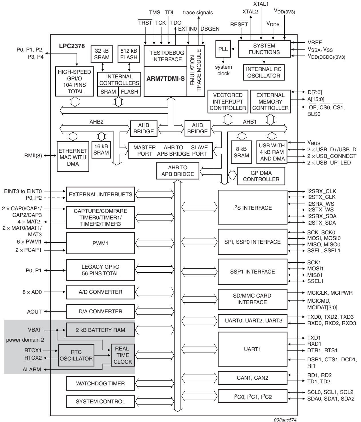
Fig 1. LPC2378 block diagram
