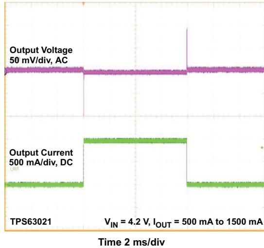
Figure 22. Load Transient Response, TPS63021
