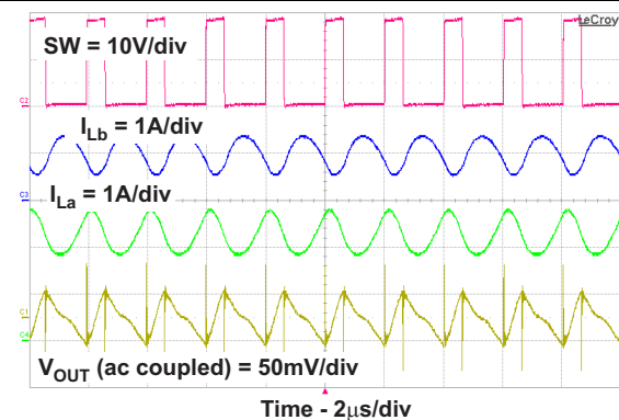
Figure 29. CCM PWM Operation
