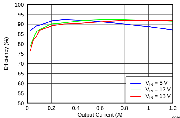
Figure 27. Efficiency vs Output Current
