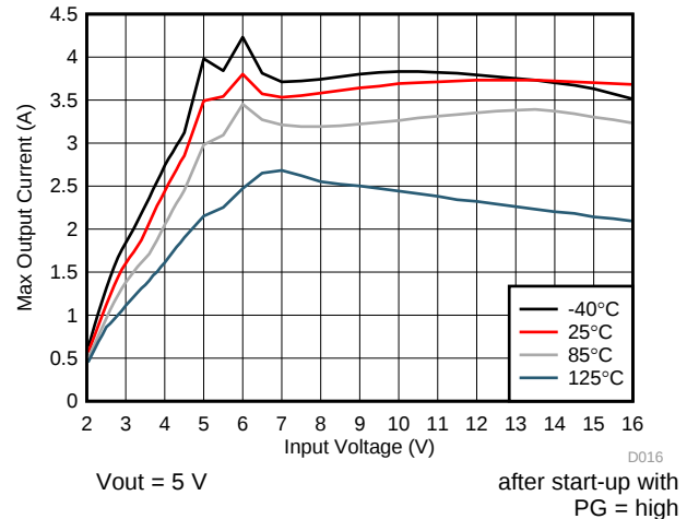
Figure 41. Maximum Load Current vs Input Voltage
