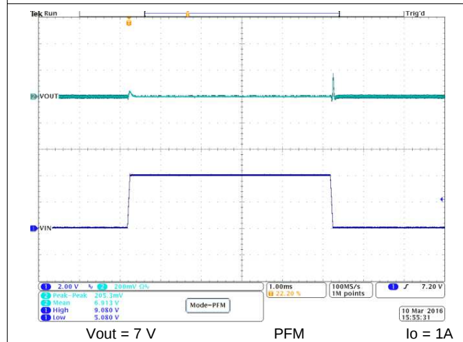
Figure 25. Line Transient Response
