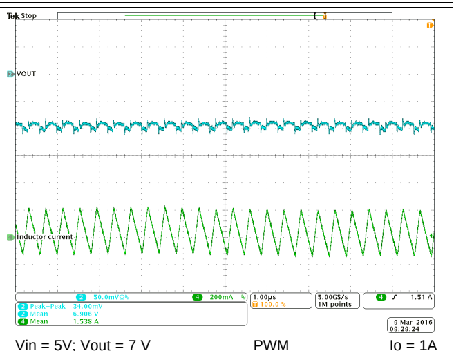
Figure 28. Output Voltage Ripple
