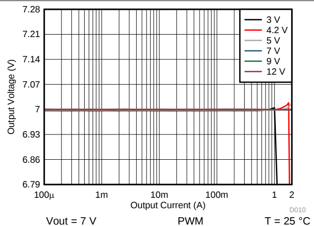
Figure 14. Output Voltage vs Output Current
