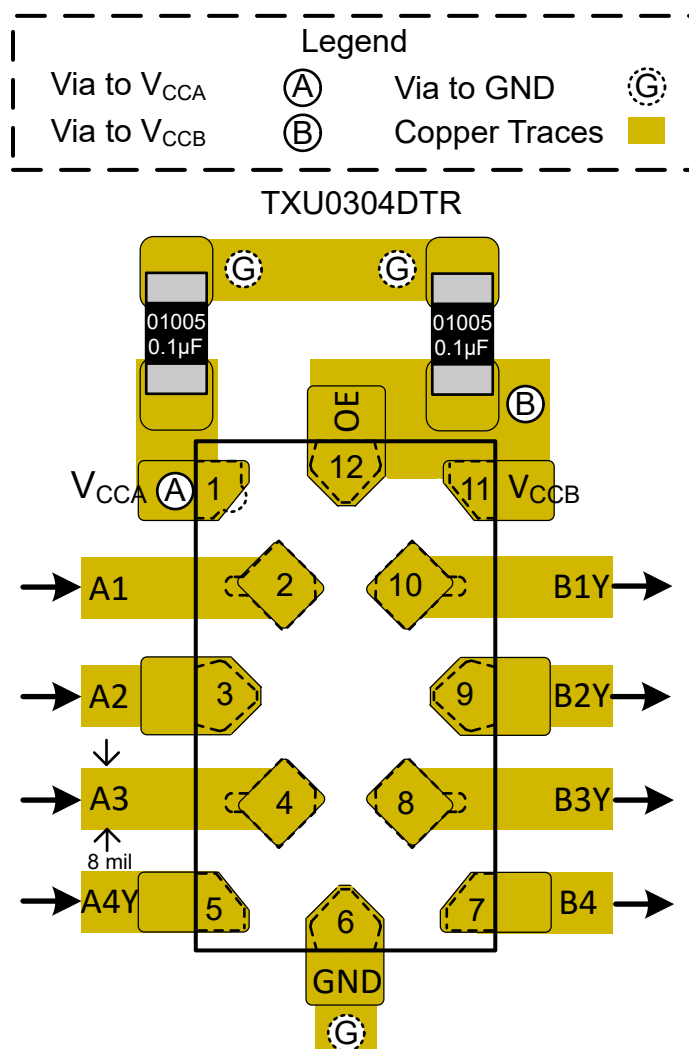
Figure 12-1. Layout Example – TXU0304
