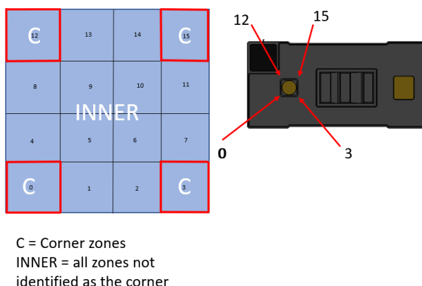
Figure 17. Zone mapping in 4x4 mode
