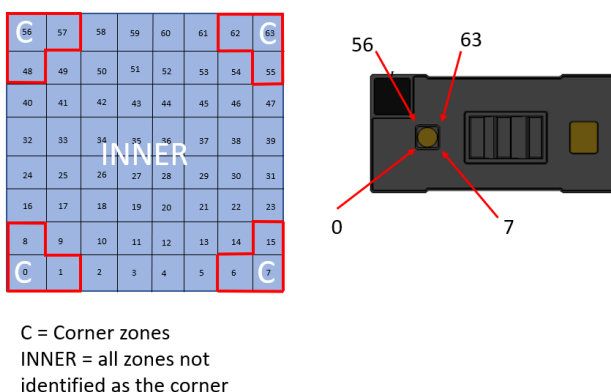
Figure 18. Zone mapping in 8x8 mode
